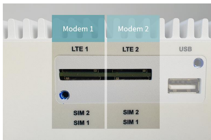
Figure 5 SIM Slot Assignment per Modem
